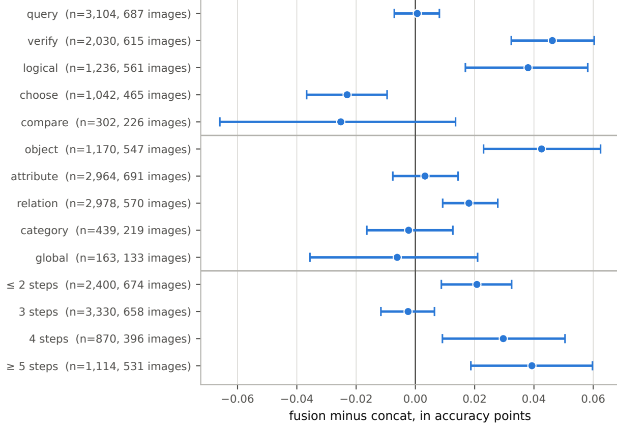
(b) fusion minus concat by slice, five-seed convention
