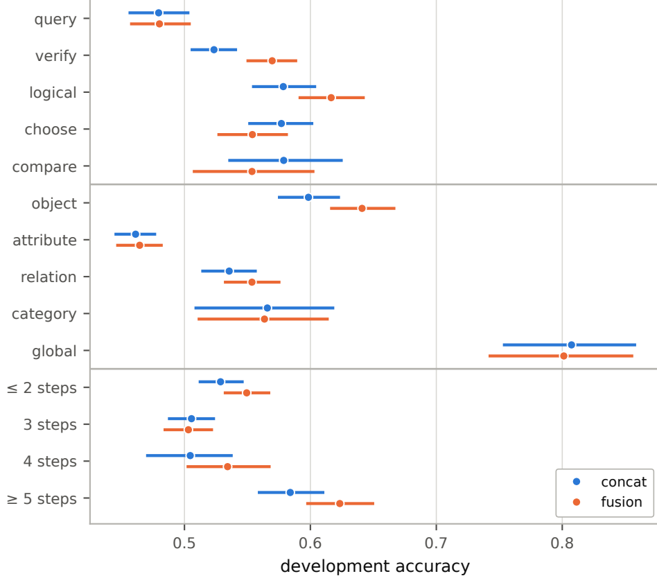
(a) per-slice accuracy at train_40k
